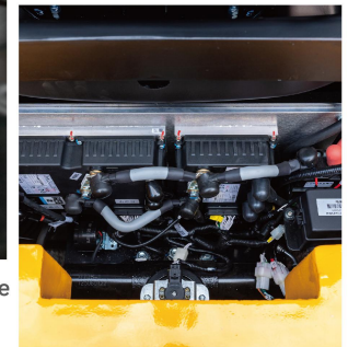
Fully opening electrical control cover for easy maintenance of electric controls and fuses.
